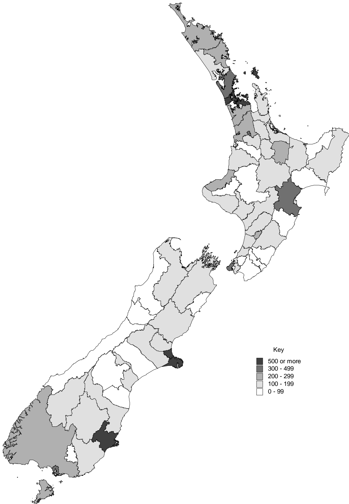
Figure 28 2005 Total Casualties
