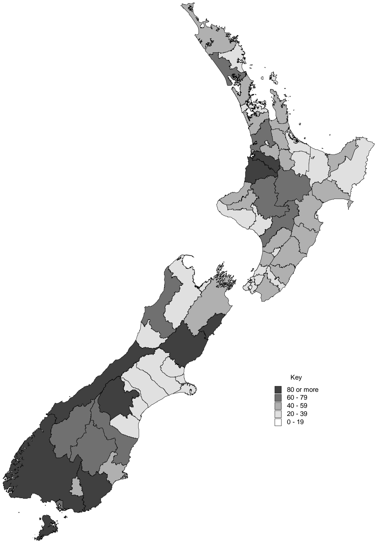
Figure 29 2006 Casualties per 10,000 Population
