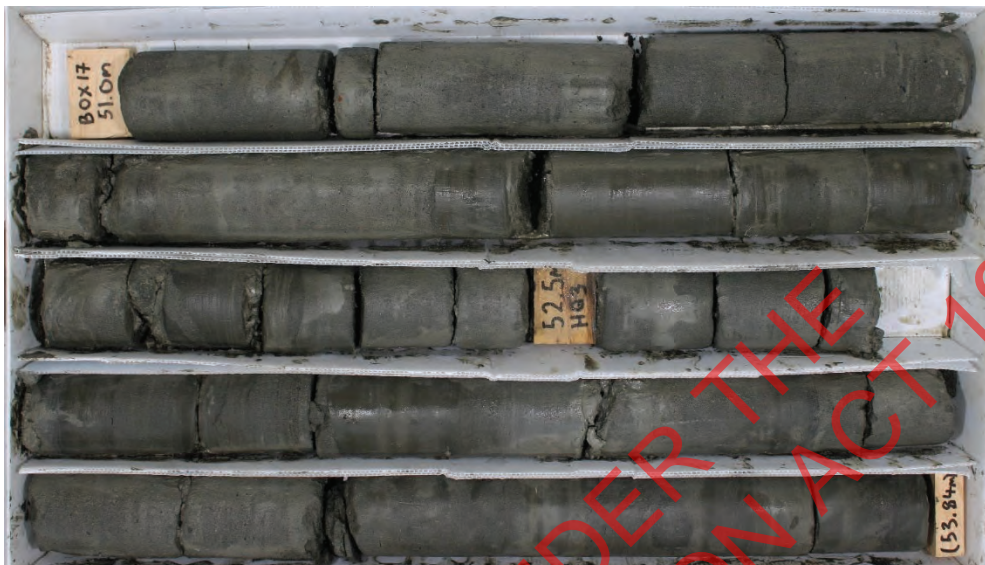
Box 17 – Depth: 51.00 to 53.84m
